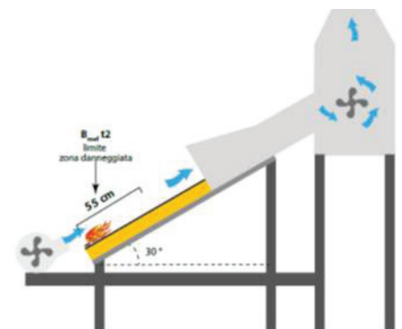
B_{roof}(t2) : equipment and test method
