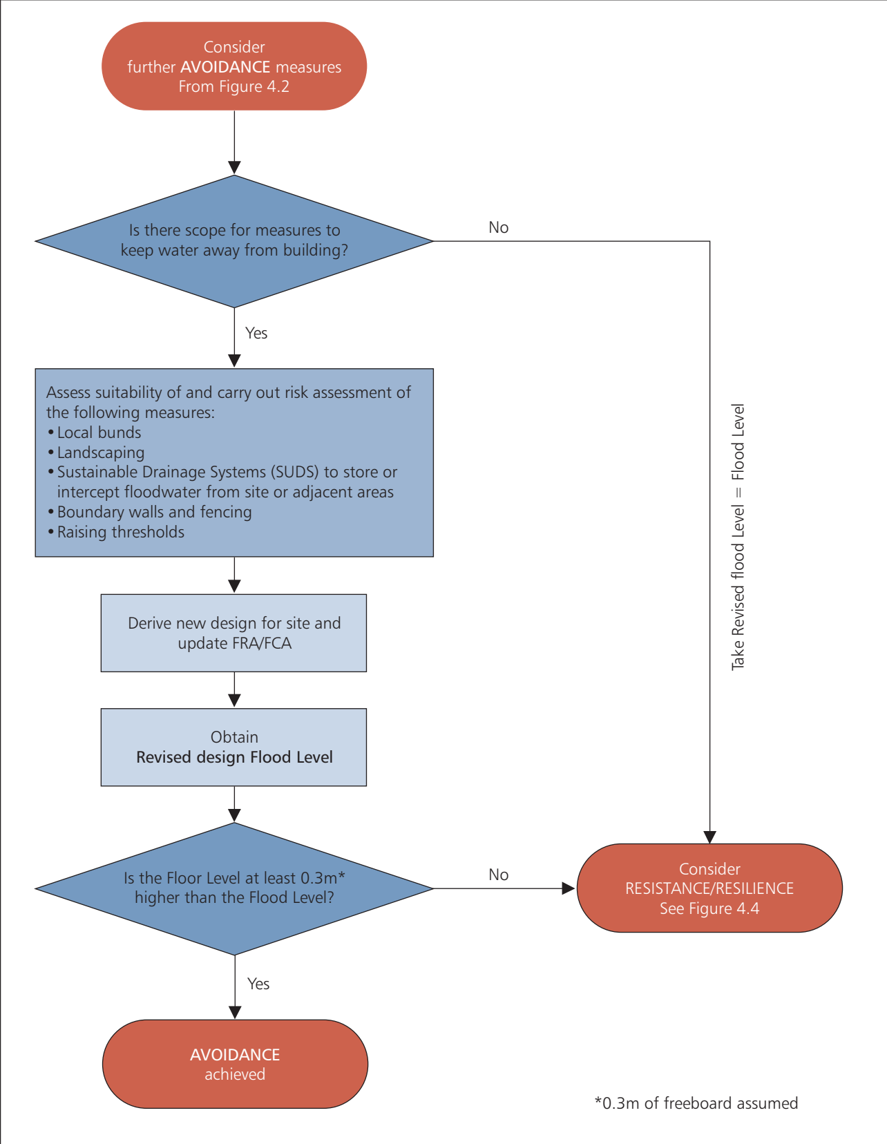
Figure 4.3 Design strategies; decision flowchart – Avoidance (2)
